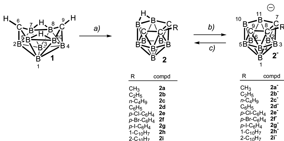
Scheme 1. Tricarbollide Compounds from the SAC Cross-Coupling via Incorporation of the RC Unit into the Structure of arachno -6,9- \text{C}_2\text{B}_8\text{H}_{14} ( 1 ) (B = BH, C = CH or C) a-c
