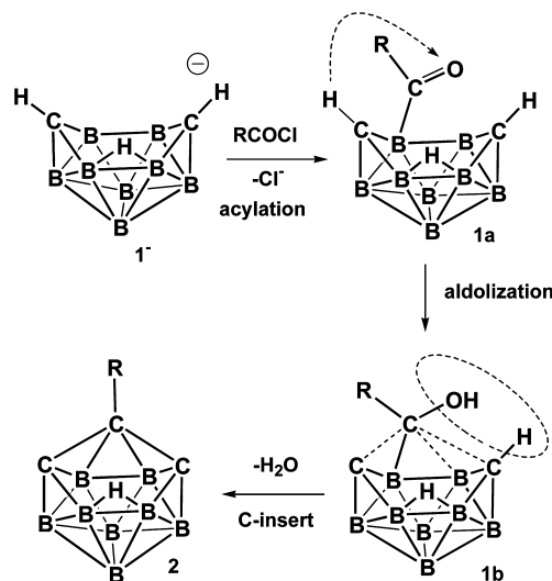
Scheme 2. Proposed Aldolization Mechanism for the Insertion of the Acyl Chloride RC Unit between the C6 and C9 Positions in [\textit{arachno}\text{-}6,9\text{-}\text{C}_2\text{B}_8\text{H}_{13}]^- ( 1 - ) (B = BH, C = CH or C)
