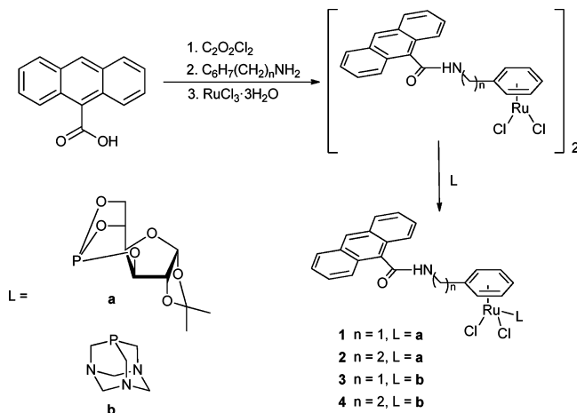
Scheme 1. Synthesis of 1–4 (a, 3,5,6-Bicyclopophosphate-1,2- O -isopropylidene- \alpha -D-glucufuranoside; b, 1,3,5-Triaza-7-phosphatricyclo[3.3.1.1]decane)
