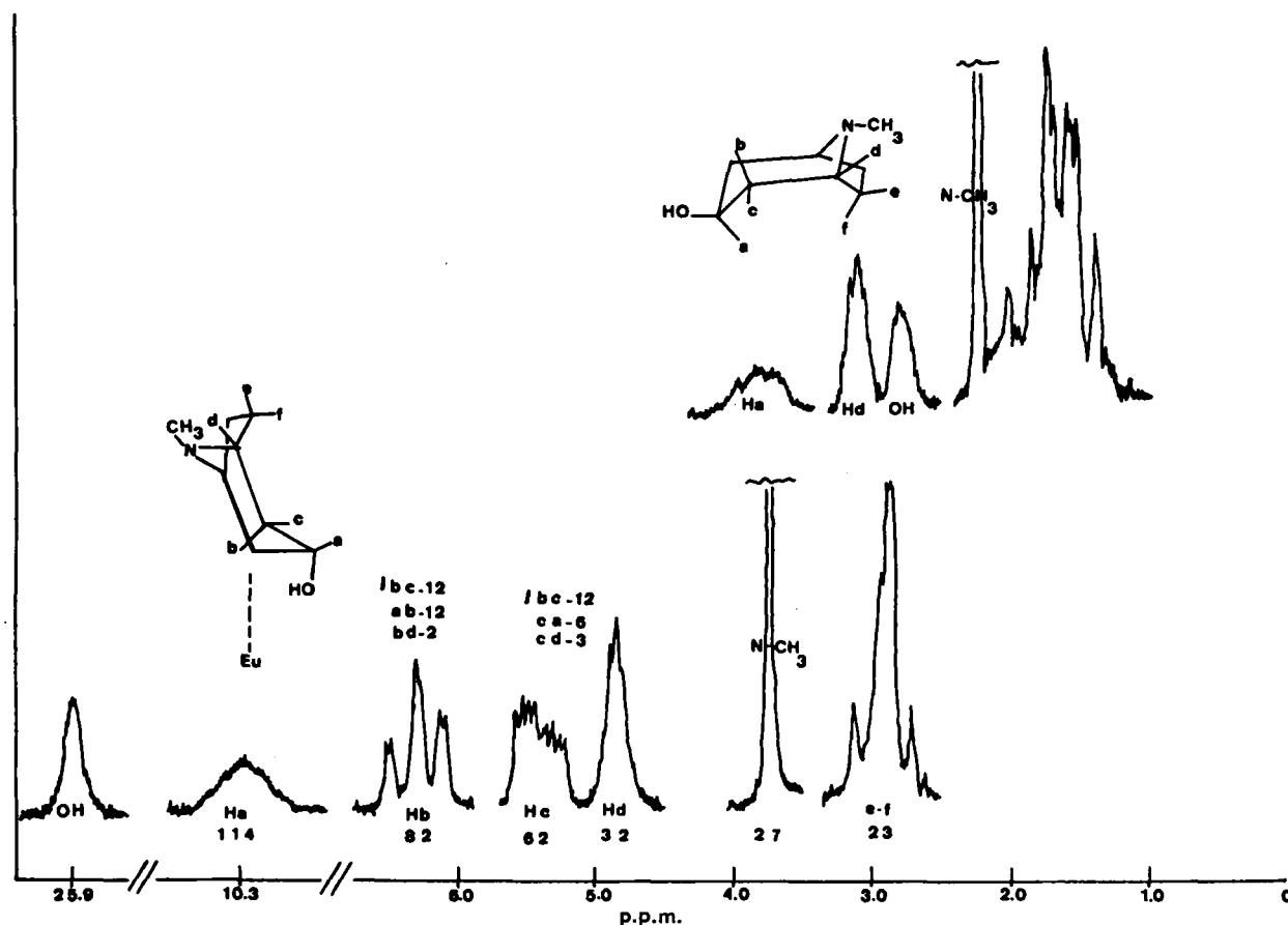
Figure 1—Pseudotropine (II) at 60 MHz, in deuteriochloroform. Key: top, without I treatment; and bottom, shifted spectra resulting at 0.35 mole ratio I/II. Numbers immediately below proton assignments represent the relative rates of proton shift between 0.2 and 0.8 mole ratio ( \Delta\delta \times 10^1 ). The alignment with the europium complex and the conformation indicated in the molecular diagram are discussed in the text.
