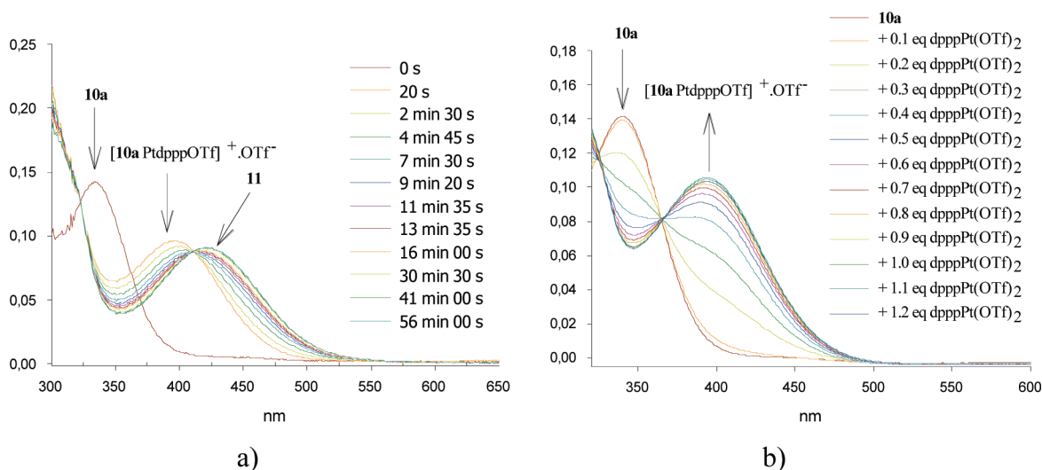
FIGURE 3. (a) Stepwise formation of 11 monitored by UV–vis spectroscopy (mixture of 10a ( 5 \times 10^{-5} mol L -1 ) in CH 3 CN with 0.5 equiv of dppp Pt(OTf) 2 ). (b) Formation of the monosubstituted complex (mixture of 10a ( 5 \times 10^{-5} mol L -1 ) in CH 3 CN with dppp Pt(OTf) 2 (0–1.2 equiv)).
