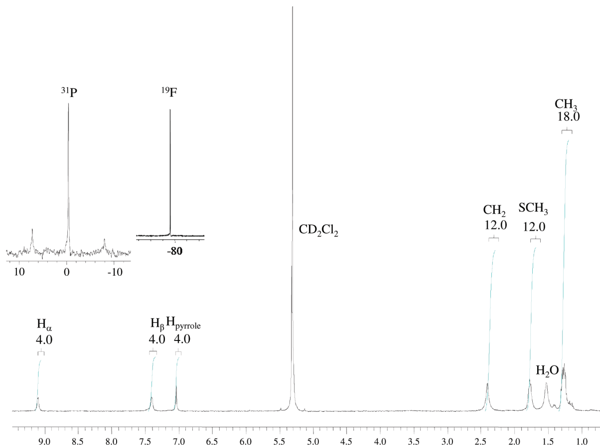
FIGURE 2. 1 H, 31 P, and 19 F NMR spectra of 13 (5 × 10 −3 mol L −1 ) in CD 2 Cl 2 .
