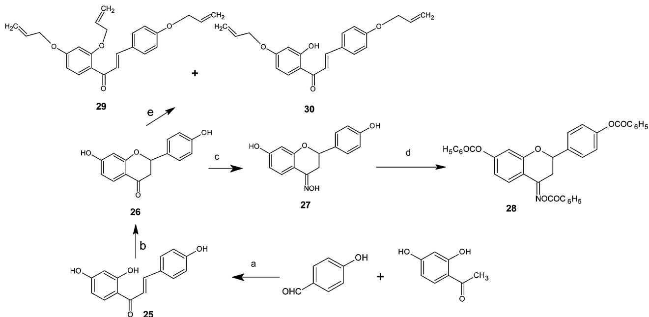
Scheme 2 Reagents and conditions: (a) 60%, aq. KOH, 100 °C, 2 h, 48%, (b) concd HCl, MeOH, reflux, 48 h, 92%, (c) \text{NH}_2\text{OH} \cdot \text{HCl} , \text{CH}_3\text{COONa} , EtOH, reflux; (d) pyridine, benzoyl chloride acetone, (e) allyl bromide, \text{K}_2\text{CO}_3 , reflux.
