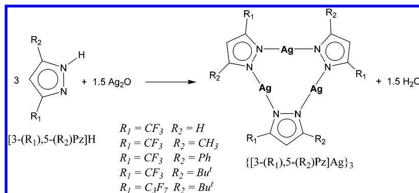
Figure 2. Synthetic route to silver pyrazolates using \text{Ag}_2\text{O} as the silver source.
