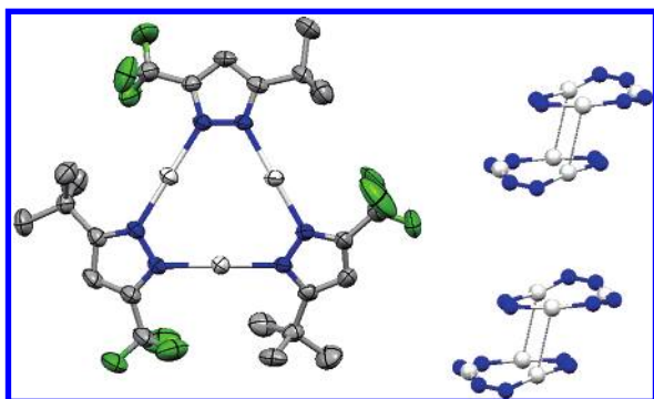
Figure 4. Molecular structure of \text{[3-(CF}_3\text{),5-(Bu}^t\text{)Pz]Ag}_3 (hydrogen atoms have been omitted for clarity) and a view showing relative arrangement of the dimers of trimers and the closest \text{Ag}\cdots\text{Ag} contacts (all except nitrogen and silver atoms have been omitted for clarity).
