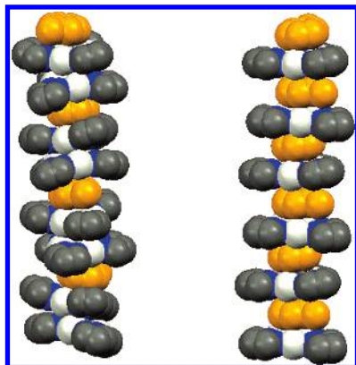
Figure 6. Sandwich structures of \{[Ag_3]_2 \cdot [toluene]\}_\infty (left) and \{[Ag_3] \cdot [3-(CF_3)_5-(Bu^t)Pz]Ag\}_3 (right): [Ag_3] = \{[3,5-(CF_3)_2Pz]Ag\}_3 and [Ag_3]' = \{[3-(C_3F_7)_5-(Bu^t)Pz]Ag\}_3 . Toluene molecules are depicted in yellow. Pyrazolyl ring substituents and hydrogen atoms have been omitted for clarity.
