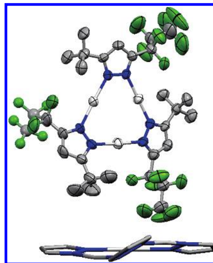
Figure 5. Molecular structure of \text{[3-(C}_3\text{F}_7\text{),5-(Bu}^t\text{)Pz]Ag}_3 (hydrogen atoms have been omitted for clarity) and a side view showing the twisted \text{Ag}_3\text{N}_6 core (pyrazolyl ring substituents have been omitted for clarity).
