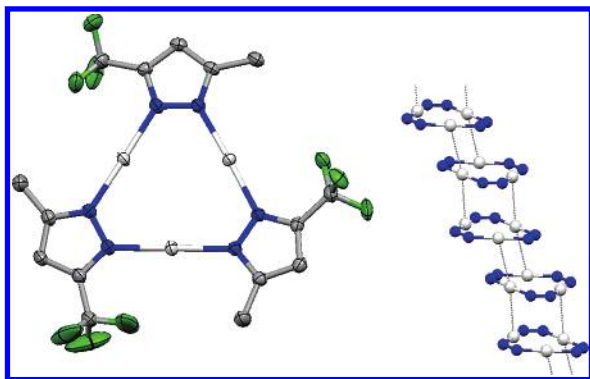
Figure 3. Molecular structure of \text{[3-(CF}_3\text{),5-(CH}_3\text{)Pz]Ag}_3 (hydrogen atoms have been omitted for clarity) and the extended chains of \text{[3-(CF}_3\text{),5-(CH}_3\text{)Pz]Ag}_3 formed via \text{Ag}\cdots\text{Ag} contacts (all except nitrogen and silver atoms have been omitted for clarity).
