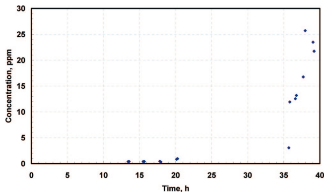
Figure 8. Breakthrough data for fixed-bed adsorption run with 1.25-h bed residence time.
