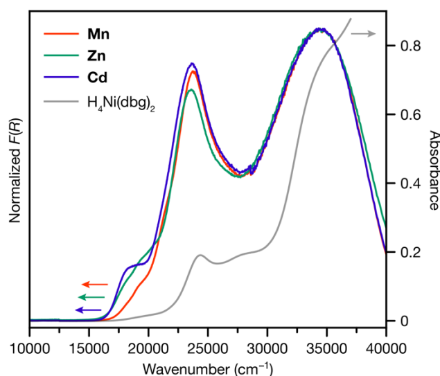
Figure 3. Kubelka–Munk-transformed diffuse reflectance UV–visible spectra of Mn , Zn , and Cd , and absorption spectrum of a 0.025 mM solution of H_4Ni(dbg)_2 in DMF.
