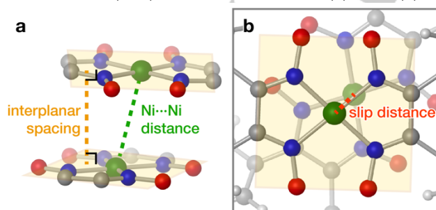
Figure 2. (a) Illustration of the interplanar and \text{Ni} \cdots \text{Ni} distances between adjacent \text{Ni}(\text{dbg})_2 linkers, with the least-squares planes shown in transparent yellow. (b) Illustration of the slip distance, defined as the projection of the \text{Ni} \cdots \text{Ni} vector onto the least-squares plane.
