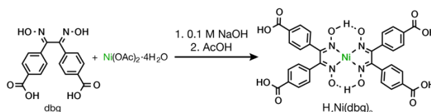
Scheme 1. Synthesis of \text{H}_4\text{Ni}(\text{dbg})_2 .
