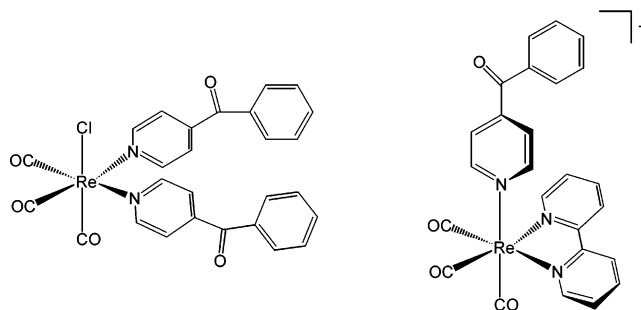
Figure 1. Schematic structures of fac -[Re(Cl)(bopy) 2 (CO) 3 ] (left) and fac -[Re(bopy)(CO) 3 (bpy)] + (right). These complexes are hereinafter denoted Re(bopy) 2 and Re(bopy)(bpy), respectively. The prefix fac will be omitted.
