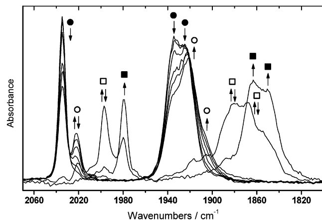
Figure 8. Low-temperature IR spectroelectrochemical reduction of Re(bpy)(bpy) measured in butyronitrile in the presence of 10 -1 M Bu 4 NPF 6 at 223 K: ●, Re(bpy)(bpy); ○, Re(bpy - )(bpy); □, Re(bpy - )(bpy - ); ■, [Re(PrCN)(CO) 3 (bpy 2- )] - .
