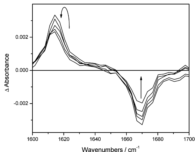
Figure 7. Time-resolved infrared spectra [\text{Re}(\text{Cl})(\text{bpy})_2(\text{CO})_3] in the region of the ketone \nu(\text{C}=\text{O}) measured in acetonitrile at 2, 4, 40, 100, and 1000 ps after 400 nm excitation. The spectra evolve in the directions of the arrows. Experimental points are separated by 4–5 \text{cm}^{-1} .
