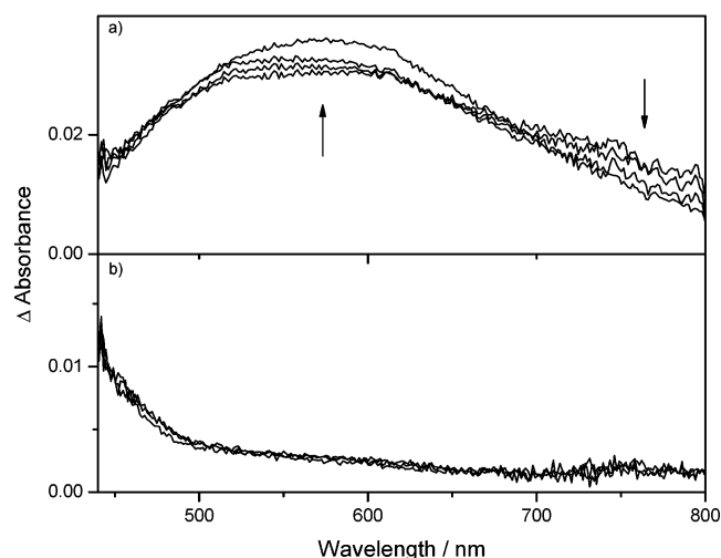
Figure 5. Time-resolved visible absorption spectra of (a) [Re(Cl)(bpy) 2 (CO) 3 ], measured at 2, 3, 10, and 75 ps, and (b) [Re(bpy)(CO) 3 (bpy)] + , measured at 4, 40, and 1000 ps. Both were measured in acetonitrile, after excitation at 393 nm. The spectra evolve in the directions of the arrows.
