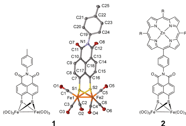
Figure 1. (left) Chemical structure of 1 . (center) X-ray structure of 1 with thermal ellipsoids set to 50% probability (see Table S1). (right) Chemical structure of 2 ( R = n\text{-C}_5\text{H}_{11} ).
