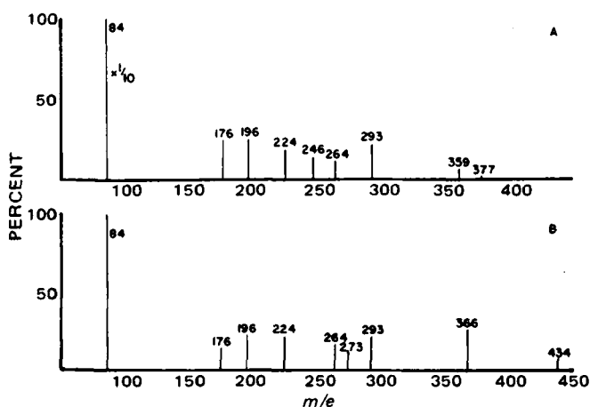
Figure 1 —Gas chromatogram-mass spectra of the free base (A) and trimethylsilyl derivative (B) of mefloquine.
