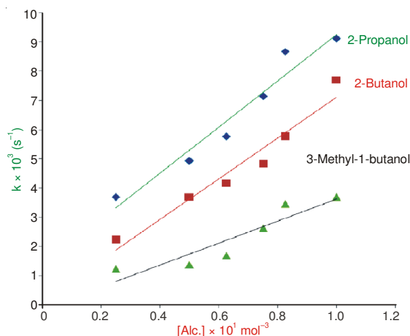
Fig. 1. Variation of rate constant of oxidation of aliphatic alcohols with [\text{Alc}]
