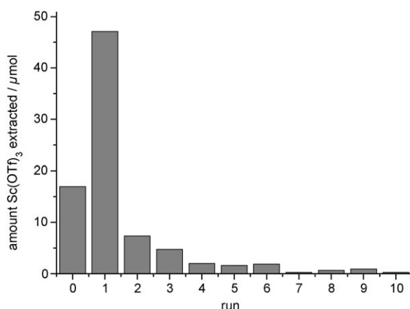
Figure 8. Results of atomic emission spectroscopy on the leaching of the catalyst from the core/shell nanofiber D prepared using 84 μmol Sc(OTf) 3 . Run 0 designates extracted Sc(OTf) 3 during the pre-washing process (30 min). For each run, the total amount Sc(OTf) 3 extracted during the reaction (3 h) and during the rinsing process (30 min) was added.
