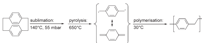
Scheme 2. Scheme of the PPX-deposition on electrospun fibers.
