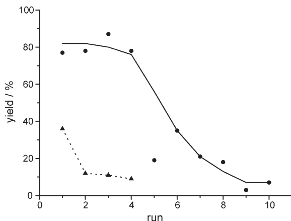
Figure 4. Dependence of the yield on the number of runs for the imino aldol reaction using catalysts A (▲) and B (●). Yields were determined by 1 H NMR spectroscopy. Diastereoisomer ratio 1.1:1.
