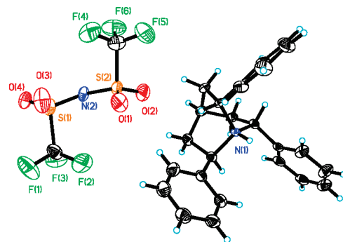
Figure 1. X-ray crystallographic structure for the salt of the (+)-enantiomer of 1 with \text{Tf}_2\text{NH} .
