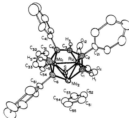
Figure 1. An ORTEP diagram of \text{RuMo}_2(\text{CO})_2(\text{C}_5\text{H}_5)_2(\mu_3\text{-S})[\mu_3\text{-}\eta^6\text{-HCC(Ph)CHC(Ph)CHC(Ph)}] (2) showing 50% probability thermal ellipsoids.
