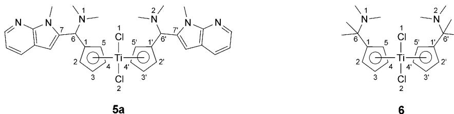
Fig. 5. Atom numbering of 5a and 6 for the structural DFT discussion of 5a
