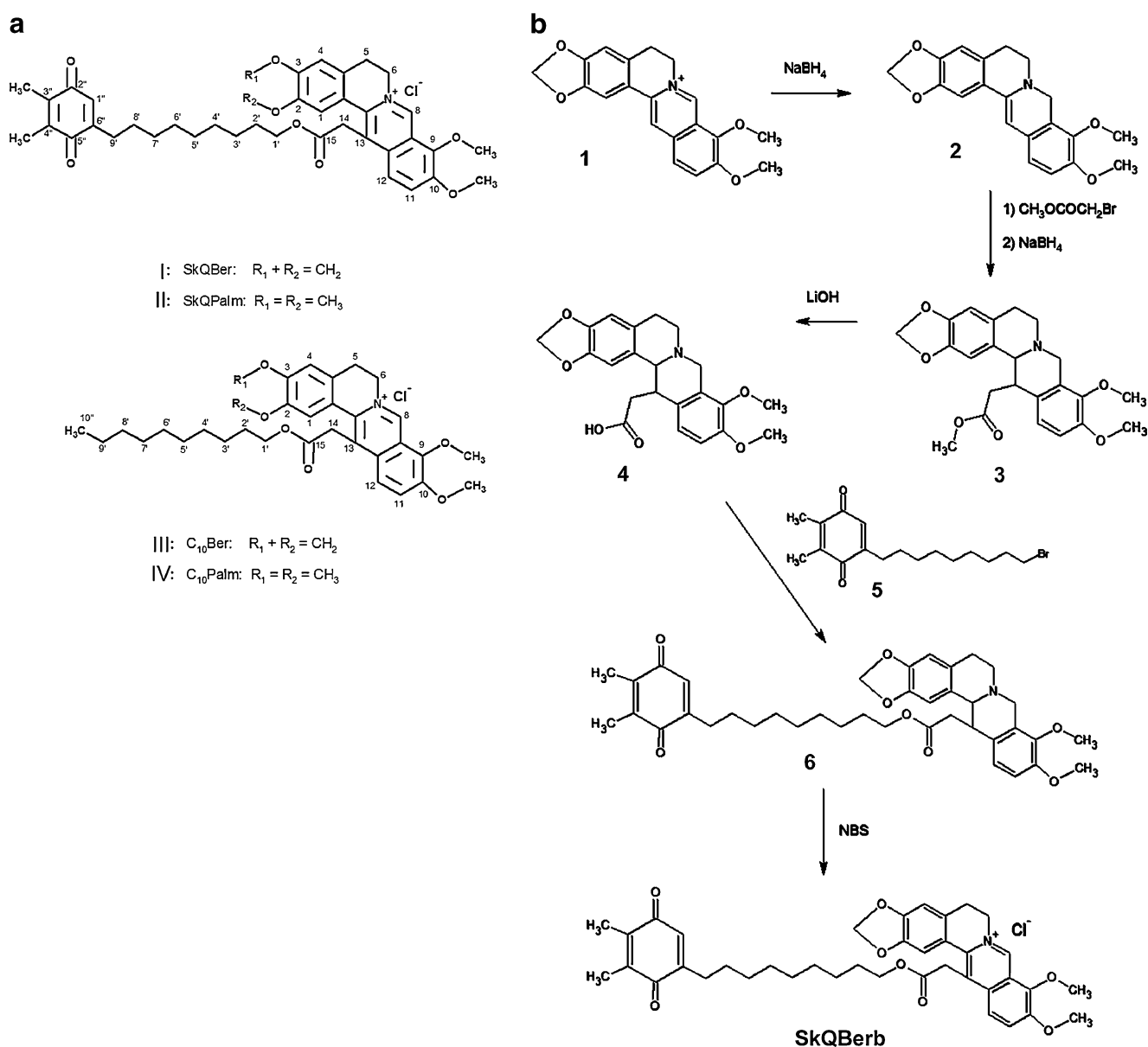
Fig. 1 Formulas of SkQBerb (I), SkQPalm (II), C 10 Berb (III), C 10 Palm (IV) ( a ) and the scheme of synthesis of SkQBerb ( b ). The same scheme was used for synthesis of C 10 Berb, SkQPalm, and C 10 Palm.
