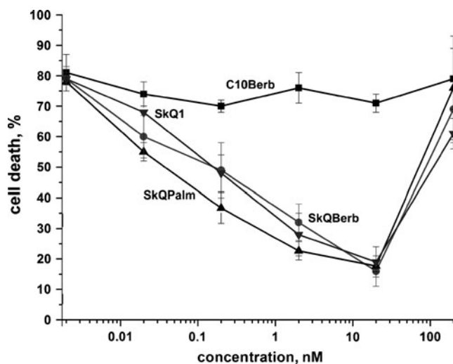
Fig. 10 SkQBerb and SkQPalm protected cells against H_2O_2 -induced damage. Fibroblasts were incubated with the antioxidants for 24 h and treated with 400 \mu M H_2O_2 for the next 24 h. Cell viability was determined with CellTiter-Blue reagent (Promega).
