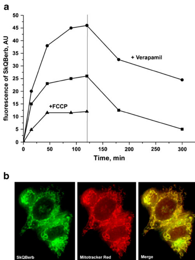
Fig. 8 Accumulation of SkQBerb in cells. (a) HeLa cells were incubated with 5 \mu M SkQBerb. 50 \mu M verapamil and 10 \mu M FCCP were added to the cells 15 min before SkQBerb. After 2 h, the medium was changed to the similar one but without SkQBerb (indicated with vertical line). Fluorescence (excitation/emission maxima, \sim 350/530 nm) was measured after detachment, washing, and lysis of the cells with detergent mixture. (b) HeLa cells were incubated with 0.5 \mu M SkQBerb for 60 min and 200 nM MitoTracker Red was added, incubated for 15 min, and analyzed with an Axiovert microscope (Carl Zeiss) equipped with a Neofluar 100 \times NA 1.3 objective.
