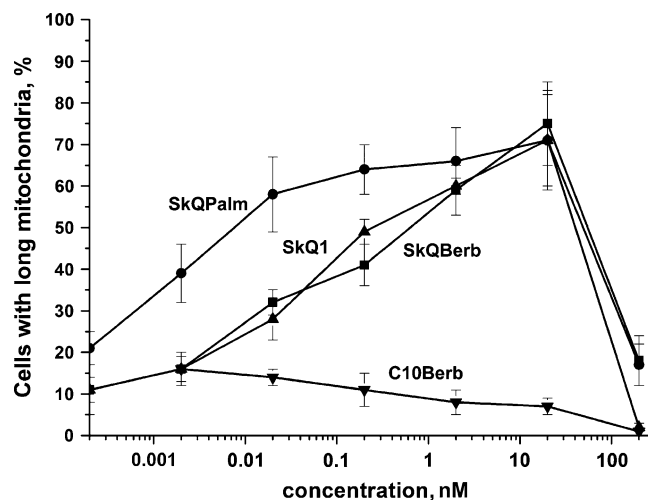
Fig. 9 SkQBerb and SkQPalm prevented fragmentation of mitochondria induced by H_2O_2 . Fibroblasts were incubated with antioxidants for 2 h and treated with 400 \mu M H_2O_2 for 3 h. Mitochondria were visualized with MitoTracker Green, and cells with elongated mitochondria were counted.
