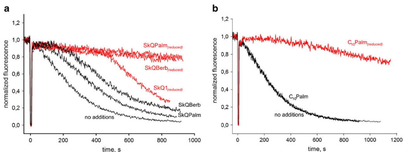
Fig. 3 Antioxidant activity of SkQBerb and SkQPalm ( a ) and C10Palm ( b ) in phosphatidylcholine/cardiolipin liposomes. All the tested compounds were added at 2 \mu\text{M} concentration. Lipid oxidation was induced by azo-initiator AMVN added at zero time and monitored as a decrease in fluorescence of BODIPY 581/591 \text{C}_{11} . In certain cases, the tested compounds were pretreated by \text{NaBH}_4 which reduced the plastoquinone as well as the berberine and palmatine moieties of the studied compounds (red curves).
