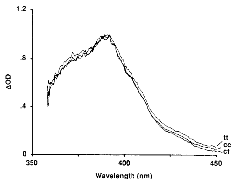
Figure 7. Triplet–triplet absorption spectra obtained by energy transfer to tt , cc , or ct , following initial excitation of 9-fluorenone. Spectra were collected 1 \mu\text{s} after the 7-ns laser pulse and are shown scaled to the same maximum absorption.
