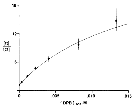
Figure 6. Photostationary tt/ct ratios obtained by sensitization with 9-fluorenone as a function of starting [ct] . The abscissa is labeled as total [DPB] because the triplet isomerization of ct gives only tt . The curve is a least-squares fit to eq 15; see text for details.
