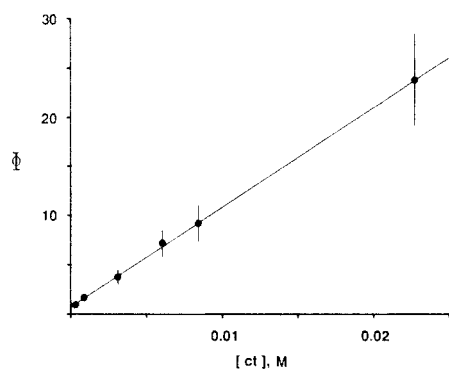
Figure 5. Initial quantum yields of ct \rightarrow tt photoisomerization by sensitization with 9-fluorenone as a function of [ct] . Quantum yield values correspond to low conversions (10–20%) and are corrected for the back reaction. The straight line is a linear least-squares fit to eq 14.
