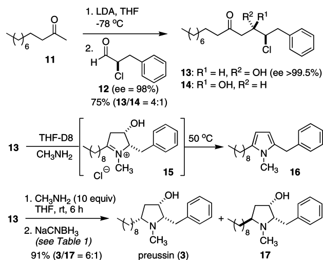
Scheme 2. Enantioselective Synthesis of (+)-Preussin ( 3 )
