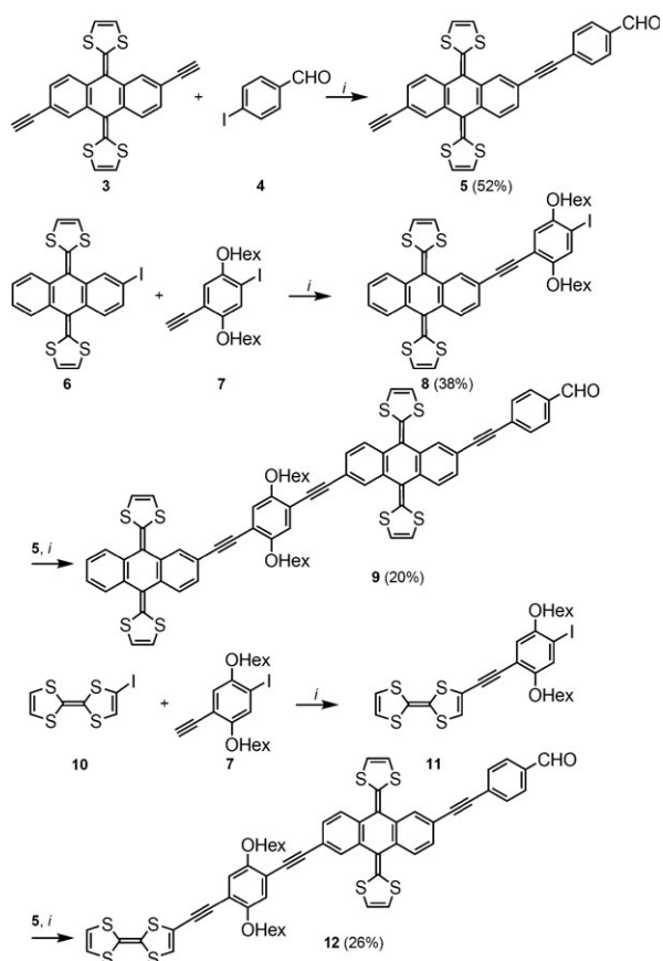
Scheme 1 Reagents and conditions used in the synthesis of 1 and 2 : (i) \text{Pd}(\text{PPh}_3)_4/\text{CuI}/i\text{Pr}_2\text{NH}/\text{THF}/\Delta .
