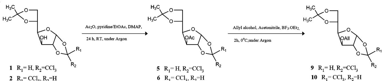
Fig. 1. Synthesis of 3- O -allyl ether derivatives of \alpha -chloralose ( 9 ) and \beta -chloralose ( 10 )
