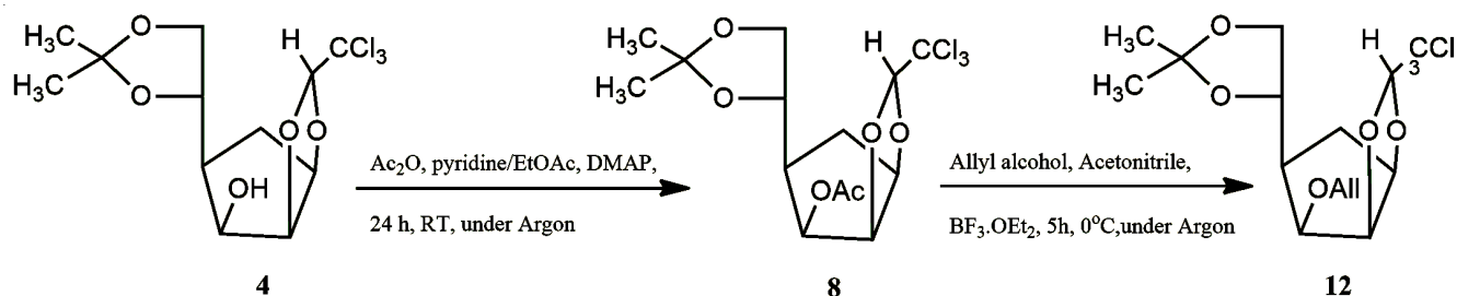
Fig. 3. Synthesis of 3- O -allyl ether derivatives of mannochloralose ( 12 )
