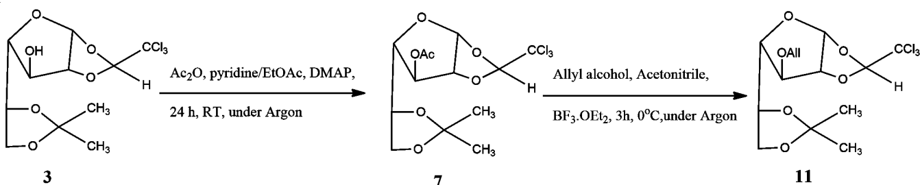
Fig. 2. Synthesis of 3- O -allyl ether derivatives of galactochloralose ( 11 )
