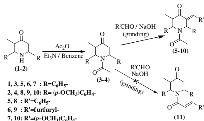
Scheme-I: Synthetic pathway of target compounds
