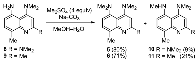
Scheme 2. Methylation of 5-Amino-4-dimethylaminoquinolines 8 and 9
