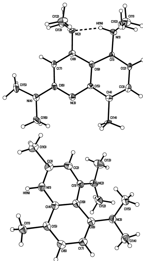
Figure 1. Molecular structures of ammonium-type 5H + ·A (above) and quinolinium-type cations 6H + ·B (below) (picrate anions are omitted for clarity; thermal ellipsoids drawn at the 50% probability level).
