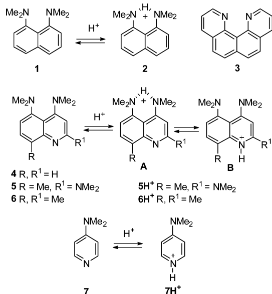
Scheme 1. Naphthalene Proton Sponge 1 , 4-Dimethylamino-pyridine 7 , and Their Quinoline Analogues 3–6
