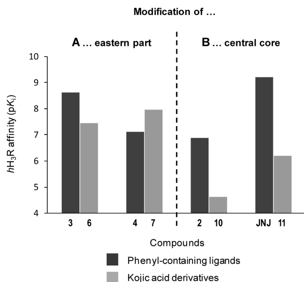
Fig. 3. Comparison of Phenyl and Pyran-4-one Moieties in the Eastern Part (A) and in the Central Core (B) of H 3 R Ligands
