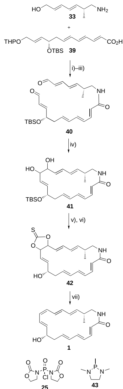
Scheme 9. Synthesis of (9 S , 18 R )-cyclamenol by means of pinacolisation and subsequent olefin formation as the key steps. i) 25 \text{NEt}_3 , THF, DMAP \rightarrow 39b , 75 %; ii) PPTS, i\text{PrOH} ; 55^\circ\text{C} , \rightarrow 39c , 73 %; iii) NMO, n\text{Pr}_4\text{RuO}_4 , 3 Å MS, \text{CH}_2\text{Cl}_2 , RT, 78 %; iv) \text{VCl}_3\cdot(\text{THF})_3 , Zn, THF, 12 h, high dilution, RT, 60 %; v) \text{CSCl}_2 , DMAP, \text{CH}_2\text{Cl}_2 , 0^\circ\text{C} , \rightarrow 41b , 65 %; vi) TBAF, HOAc, THF, RT, 26 %; vii) 43 , \text{Et}_2\text{O} , -20^\circ\text{C} , 20 %.
