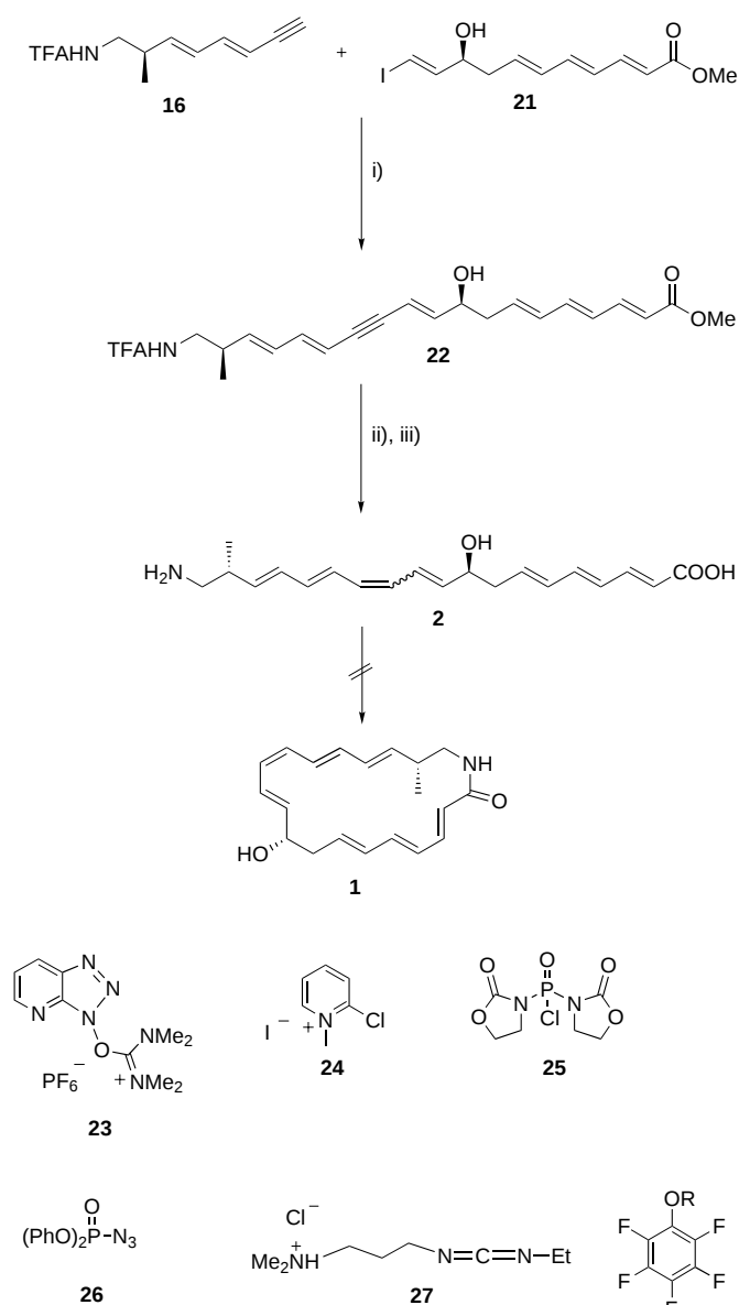
Scheme 5. Attempted synthesis of target compound 1 by macrolactamisation as final ring-closing step. i) \text{Pd}(\text{PhCN})_2\text{Cl}_2 , \text{CuI} , piperidine, \text{PhH} , 87 %; ii) \text{Zn}(\text{Cu}/\text{Ag}) , \text{MeOH} \rightarrow 22b , 55 %; iii) \text{LiOH} , \text{THF}/\text{MeOH}/\text{H}_2\text{O} , 40 %.
