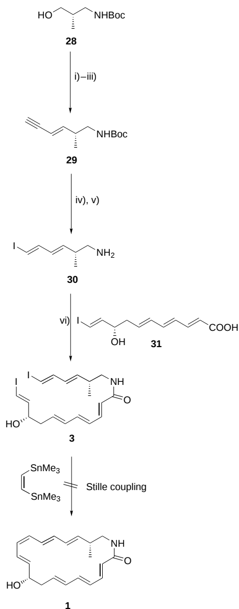
Scheme 6. Attempted synthesis of target compound 1 by double Stille coupling as final ring-closing step. i) (COCl) 2 , DMSO, NEt 3 ; ii) 9 , n BuLi, THF, → 28b , 72%, two steps; iii) K 2 CO 3 , MeOH, 93%; iv) Cp 2 ZrCl 2 /LiBEt 3 H then I 2 , → 29b , 75%; v) TMSOTf, lutidine, 90%; vi) (EtO) 2 -POCN, NEt 3 , DMF, 74%.
