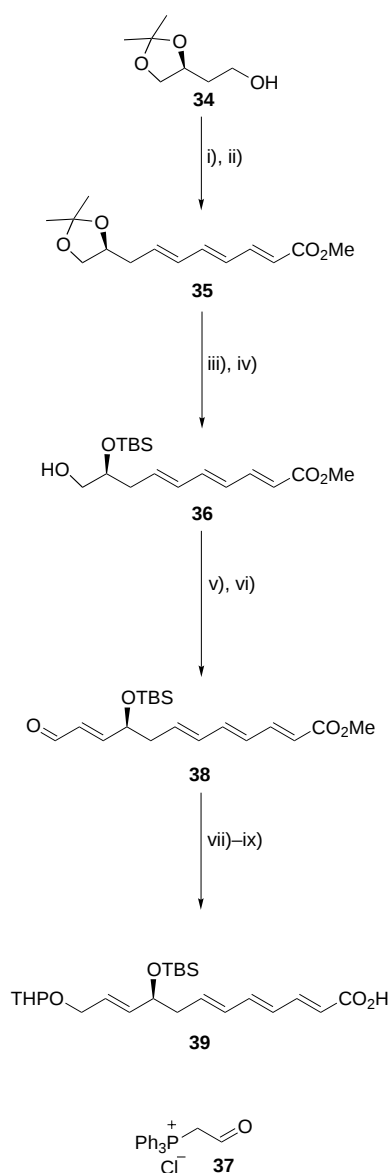
Scheme 8. Synthesis of advanced building block 39 from selectively protected triol 34 . i) (\text{COCl})_2 , DMSO, \text{CH}_2\text{Cl}_2 , -78^\circ\text{C} , \text{NEt}_3 ; ii) 7 , n\text{BuLi} , THF, 0^\circ\text{C} to RT, 85 % for two steps; iii) \text{TosOH} ; MeOH, RT, then TBSCl, imidazole, DMF, \rightarrow 35b , 82 %; iv) \text{HF}\cdot\text{py} , pyridine, THF, RT, 73 %; v) (\text{COCl})_2 , DMSO, \text{CH}_2\text{Cl}_2 , -78^\circ\text{C} , \text{NEt}_3 ; vi) 37 \text{NEt}_3 , \text{CH}_2\text{Cl}_2 , RT, 70 % for two steps; vii) \text{CeCl}_3\cdot 7\text{H}_2\text{O} , \text{NaBH}_4 , i\text{PrOH} , 0^\circ\text{C} , \rightarrow 38b , 77 %; viii) PPTS, DHP, \text{CH}_2\text{Cl}_2 , RT, \rightarrow 38c , 93 %; ix) \text{LiOH}\cdot\text{H}_2\text{O} , THF/MeOH/ \text{H}_2\text{O} , 72 %.
