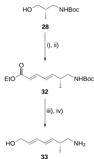
Scheme 7. Synthesis of advanced building block 33 from selectively protected amino alcohol 28 . i) (COCl) 2 , DMSO, NEt 3 ; ii) 10 , LDA, –78 °C to RT, 83% for two steps; iii) DIBAL; CH 2 Cl 2 , –78 °C to –30 °C, → 32b , 90%; iv) TFA/CH 2 Cl 2 3:5, 0 °C, then aq. K 2 CO 3 , 84%.
