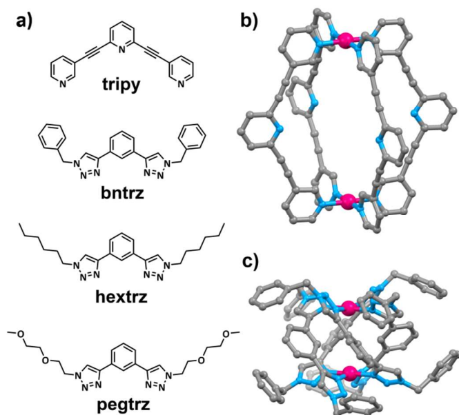
Figure 1 a) Chemical structures of the pyridine- ( tripy ) and triazole- ( bntrz , hextrz and pegtrz ) based ligands; the molecular structures of b) [Pd 2 ( tripy ) 4 ](BF 4 ) 4 26 and c) [Pd 2 ( bntrz ) 4 ](BF 4 ) 4 24h architectures. Anions, solvent molecules and hydrogen atoms have been omitted for clarity.
