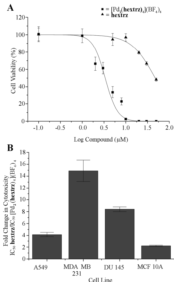
Figure 2. [Pd_2(\text{hextrz})_4](BF_4)_4 cytotoxicity is not due to helicate decomposition. Cells were treated with [Pd_2(\text{hextrz})_4](BF_4)_4 or hextrz for 24 hours before cell viability analysis. (A) Against DU-145 cells the IC_{50} for the ligand (28.5 \mu M ) was 8 fold higher than for the helicate (3.4 \mu M ); if helicate toxicity was due to rapid decomposition to release the ligand, then the stoichiometry of the complex would predict a 4-fold ratio in IC_{50} . (B) A comparison of the IC_{50} ratio between ligand and helicate across the four cell lines demonstrated no correlation between helicate and ligand toxicity. Data points are expressed as means \pm SEM where n=6 .
