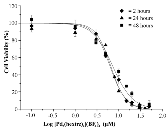
Figure 3. Cell death caused by [Pd_2(\text{hextrz})_4](BF_4)_4 occurs within 2 hours post administration. A549 cells were treated with 0-50 \mu M [Pd_2(\text{hextrz})_4](BF_4)_4 for 2, 24 or 48 hours, and cell viability assessed. There was no significant difference in IC_{50} between time points. Data are expressed as means \pm SEM ( n=6 ).
