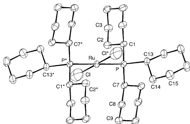
Figure 11. Molecular structure of complex 18 , anisotropic displacement parameters are drawn at 50% probability, hydrogen atoms omitted for clarity.
