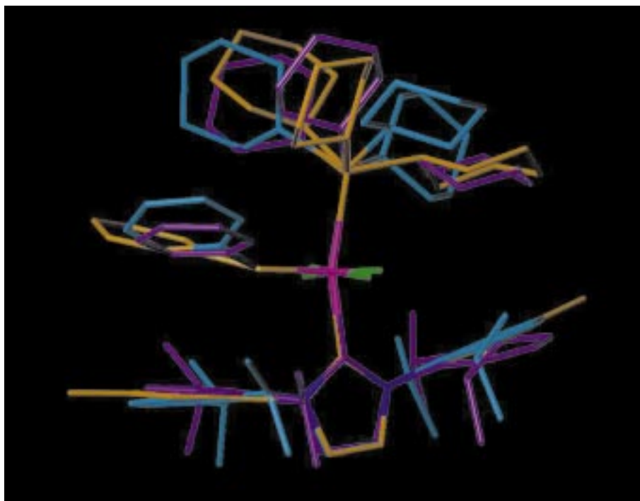
Figure 9. Superposition of the polymorphs of complex 10 using the following color code: 10a (cyan), 10b (mauve), 10c [15c] (orange).
