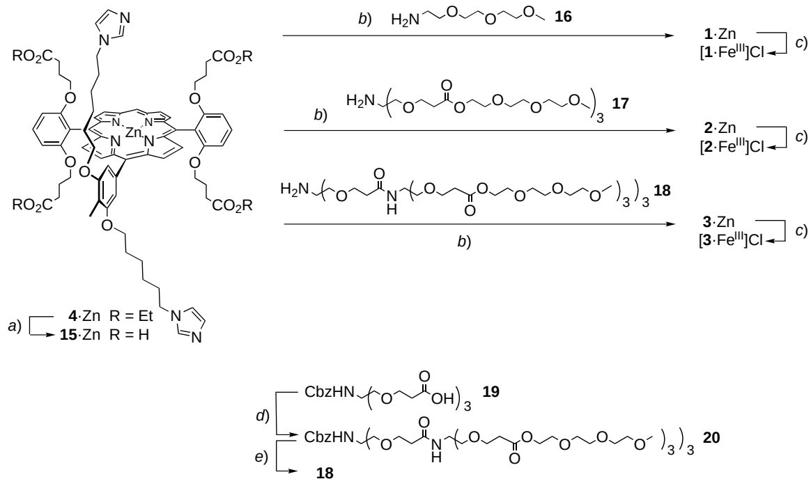
Scheme 2. Synthesis of the Dendritic Cytochrome Mimics [1 \cdot \text{Fe}^{\text{III}}]\text{Cl} , [2 \cdot \text{Fe}^{\text{III}}]\text{Cl} , and [3 \cdot \text{Fe}^{\text{III}}]\text{Cl} and the Dendritic Wedge 18
