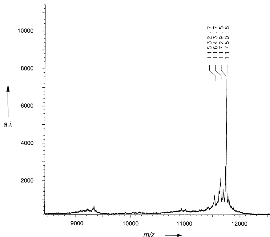
Fig. 5. MALDI-TOF Mass spectrum of the dendritic \text{Zn}^{\text{II}} porphyrin \mathbf{3} \cdot \text{Zn} . Matrix: 0.01M 2-(4-hydroxyphenyl-azo)benzoic acid (HABA) in MeCN/ \text{H}_2\text{O} 4:1, analyte in \text{CH}_2\text{Cl}_2 ; reflector mode.
