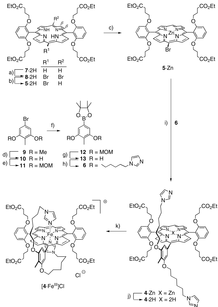
Scheme 1. Synthesis of the Bis-Imidazole-Ligated Iron(III) Porphyrin Core [4 \cdot \text{Fe}^{\text{III}}]\text{Cl}
