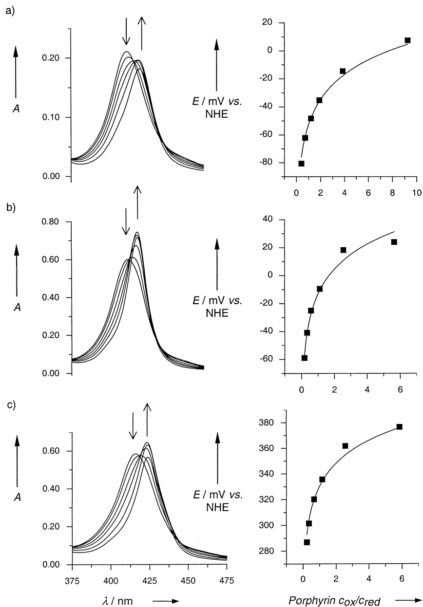
Fig. 9. Redox equilibria in H_2O between [Fe(ox)_3]^{4-/3-} and [1 \cdot Fe^{III}]Cl (a), and [2 \cdot Fe^{III}]Cl (b) and between [Fe(CN)_6]^{4-/3-} and [3 \cdot Fe^{III}]Cl (c). Spectral evolution of the Soret-band region in the UV/VIS spectrum during reductive titration (left) and nonlinear least-squares fit of the titration data to the Nernst equation, yielding the redox potential (right). A stock solution of fully oxidized porphyrin (typical concentration 5 \cdot 10^{-6} M) was titrated with a stock solution of fully reduced reference compound (typical concentration 2.5 \cdot 10^{-4} M), and the concentrations of all species in solution calculated at each titration point from the spectrophotometrically determined ratio of oxidized to reduced porphyrin and known total concentrations; T = 298 K.
