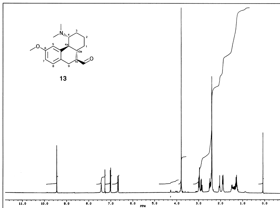
Fig. 1. ^1\text{H} -NMR Spectrum of phenanthrenecarbaldehyde 13 obtained by Friedel-Crafts substitution of the model compound 12
