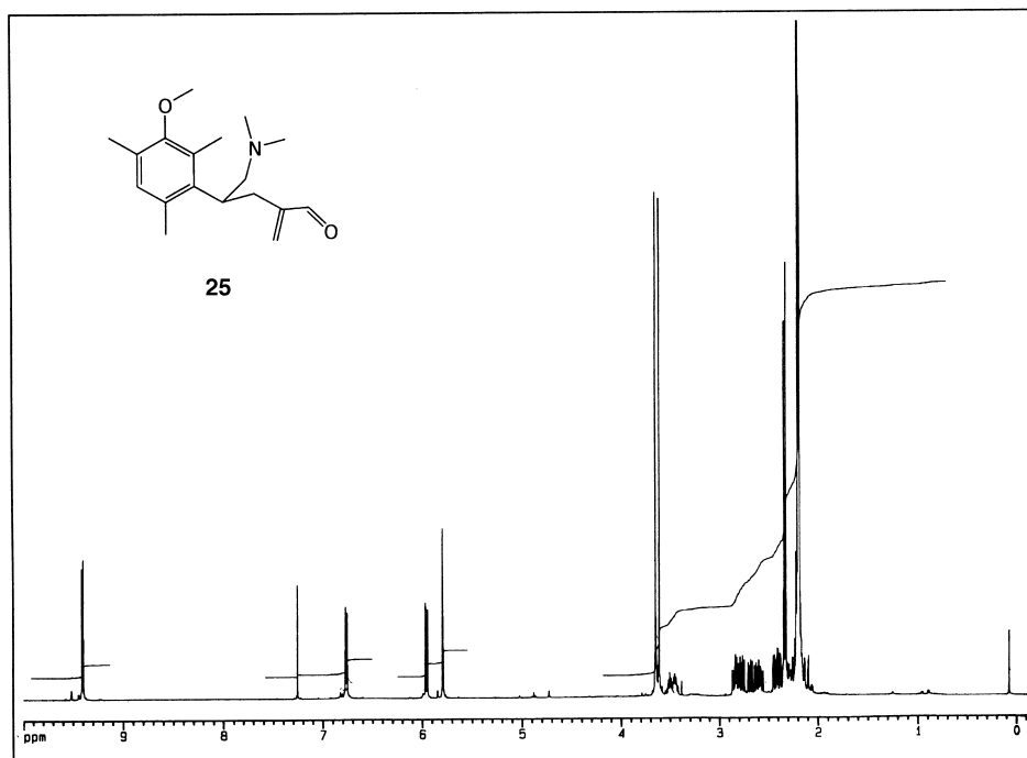
Fig. 2. ^1\text{H} -NMR Spectrum of the model compound 25
