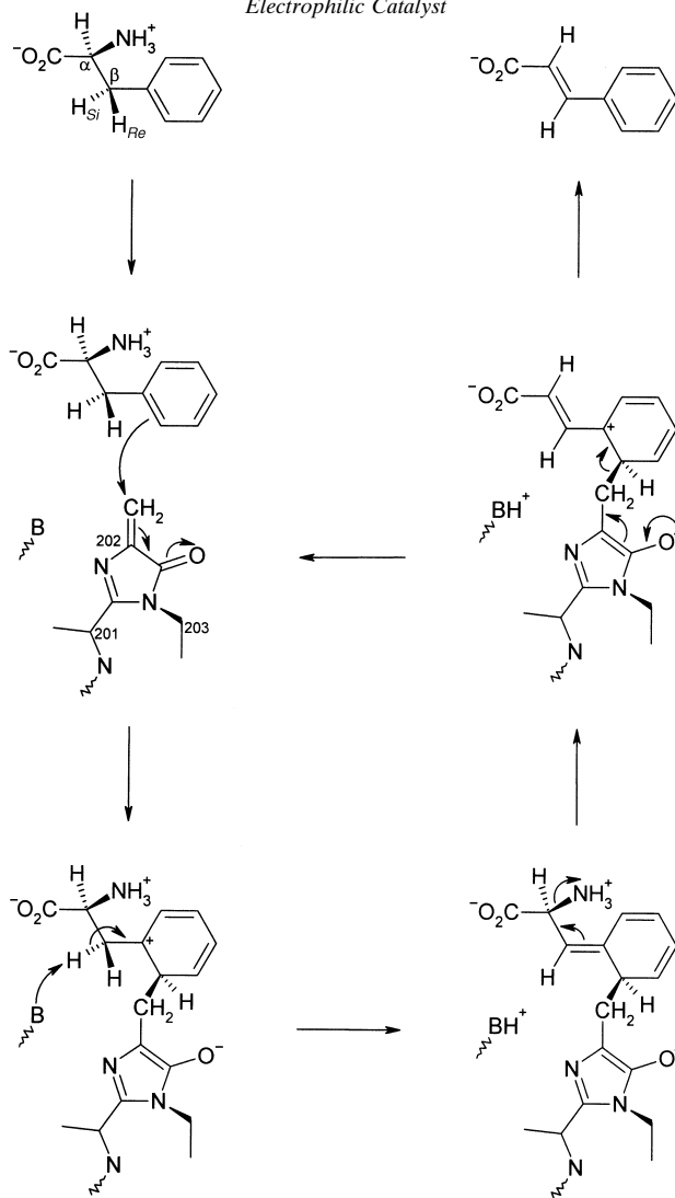
Scheme 1. Proposed Mechanism of Action of Phenylalanine Ammonia Lyase: Involvement of MIO as Electrophilic Catalyst
