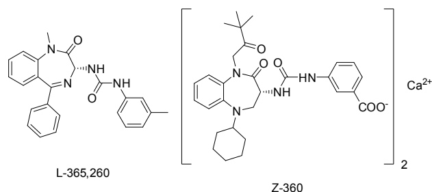
Figure 1. CCK 2 / gastrin antagonists, Merck standard and most recent addition.
