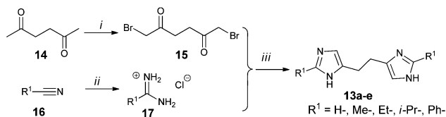
Scheme 1 Synthesis of bis[1 H -imidazol-4(5) yl ]ethane derivatives 13a–e . Reactions and conditions: (i) Br 2 , H 2 SO 4 , MeOH, 0 °C to r.t., 12 h; (ii) HCl, EtOH 0 °C to r.t., 2 h then NH 3 7 N, MeOH 4 h r.t.; (iii) NH 3 –MeOH 7 N, MW 200 W, 120 °C, 40 min.
