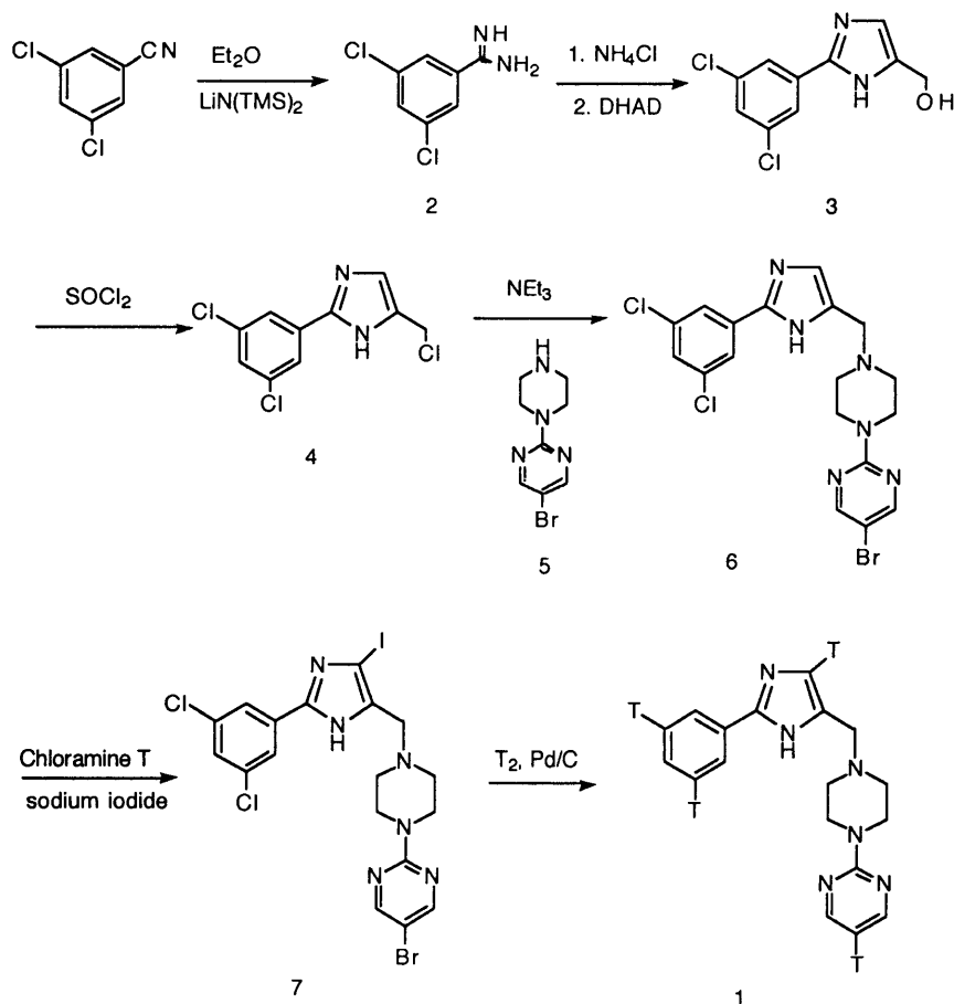
Scheme 1. Synthesis of Tritiated 2-Phenyl-4-[4-(2-pyrimidyl)piperazinyl]methylimidazole ([ 3 H]-NGD 94-1).
