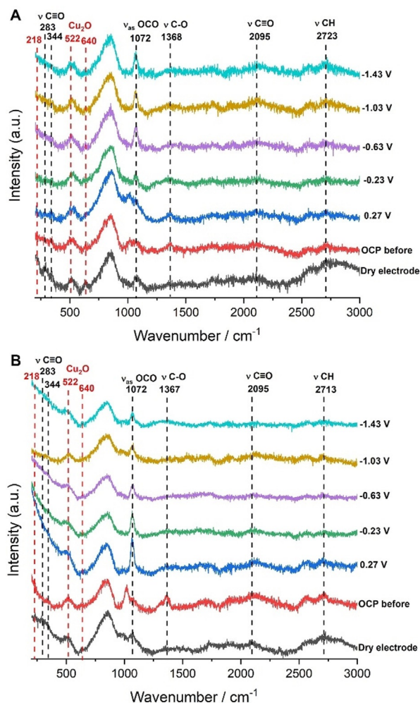
Figure 5. Operando electrochemistry Raman spectra for a) 0.5 B-Cu GDE and b) 0.5 B-Cu:0.025 Zn GDE during eCO 2 RR at different applied potentials.
