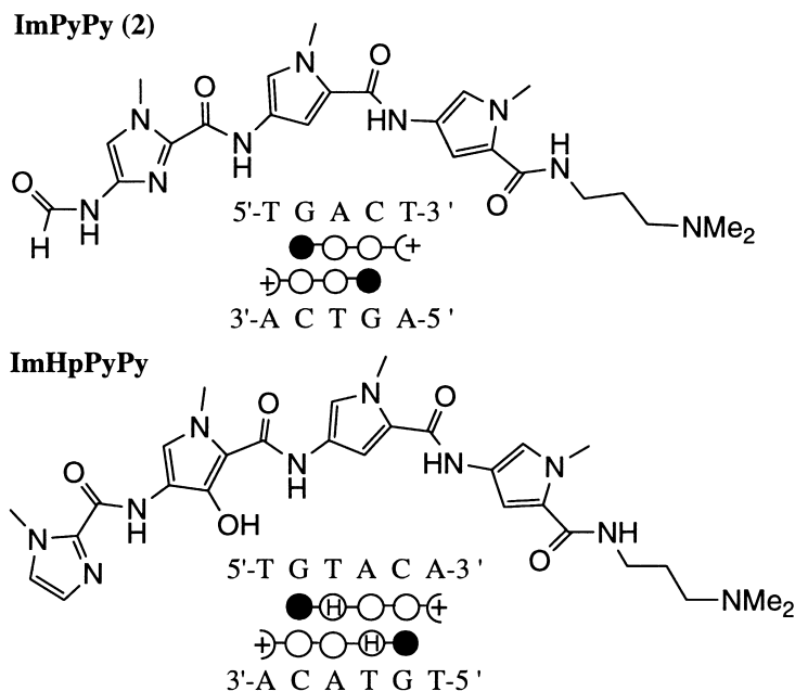
Fig. 2. Structures and 2:1 binding modes of synthetic molecules which recognize DNA in the minor groove. ImPyPy and ImHpPyPy bind 5'-TGACT-3' and 5'-TGTACA-3', respectively, as antiparallel homodimers. The pairing rules for polyamide recognition of DNA arose from study of the sequence specificity of these and similar molecules.
