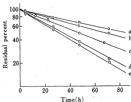
Fig. 1. First-order Plots for the Degradation of Ampicillin in the Presence and Absence of Furfural in 0.07 M Phosphate Buffer (pH 8.00) at 35°C and \mu=0.5
