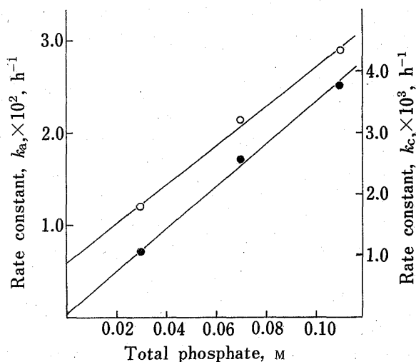
Fig. 3. Plots of Rate Constant, k_a or k_e , versus Buffer Concentration at pH 8.00
