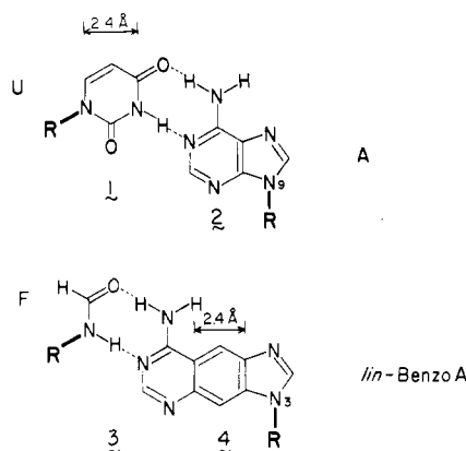
Figure 1. Base-pairing scheme of uridine (1) with adenosine (2) as compared to hypothetical base-pairing but would be 2.4 Å narrower or shorter than uridine, and thus would be a foreshortened analogue of uridine.
