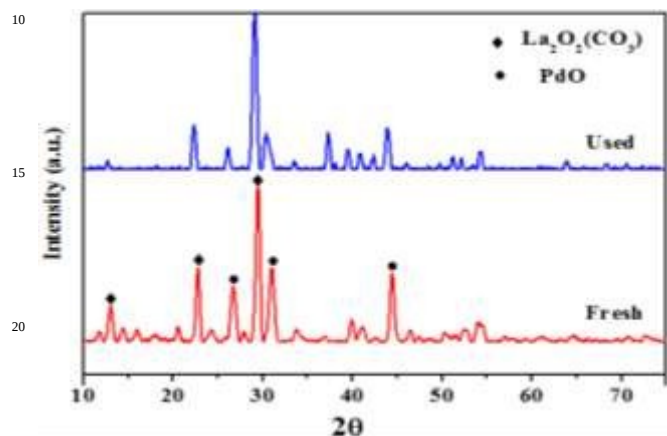
Fig. 1 XRD patterns of the Pd(II)/Mg-La mixed oxide: fresh and used catalysts
