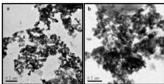
Fig. 2 TEM images of the Pd (II)/Mg-La mixed oxide: [a] fresh and [b] used catalyst (recovered after 1 st cycle).
