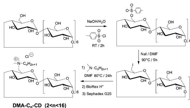
Scheme 1 Three step synthesis of DMA- C n -CDs.
