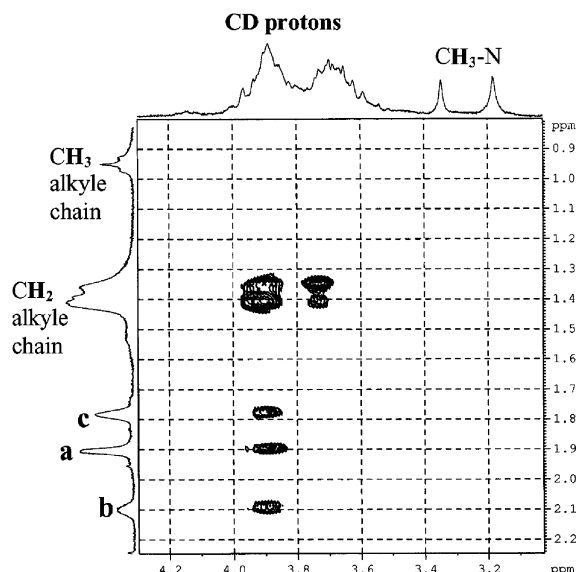
Fig. 4 2D T-ROESY data (300 ms mixing time) at 298 K in \text{D}_2\text{O} of a 1 : 1 mixture of DMA- \text{C}_{12} -CD (10 mM) and Adac (10 mM).
