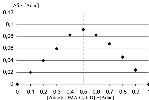
Fig. 5 Job plot upon mixing DMA- \text{C}_4 -CD and Adac. The total concentration of the two components was 1 \mu\text{M} in \text{D}_2\text{O} , with mole fractions varying from 0 to 1.
