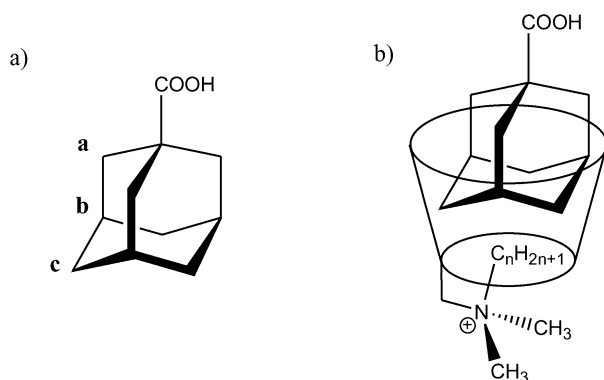
Scheme 2 (a) 1-Adamantanecarboxylic acid (Adac); (b) inclusion complex between DMA- \text{C}_n -CD ( n > 2 ) and Adac.
