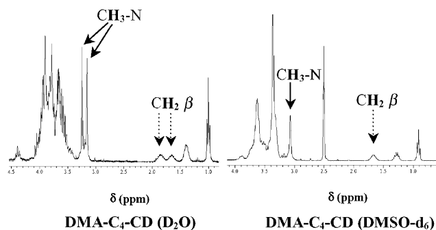
Fig. 3 Partial ^1\text{H} NMR spectra of DMA- \text{C}_4 -CD (10 mM) in \text{D}_2\text{O} and \text{DMSO-d}_6 at 298 K.
