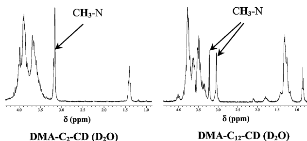
Fig. 2 Partial 1 H NMR spectra of DMA-C 2 -CD and DMA-C 12 -CD (10 mM) at 298 K in D 2 O.
