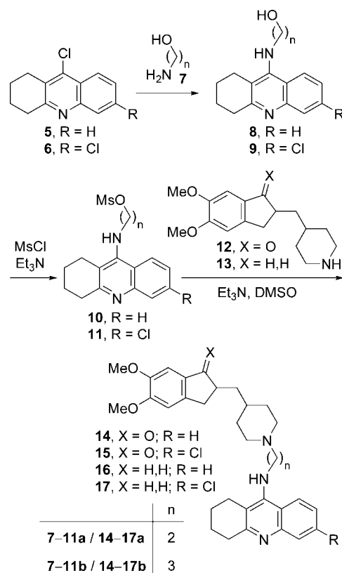
Scheme 1. Synthesis of the Donepezil-Tacrine Hybrids 14–17a,b
