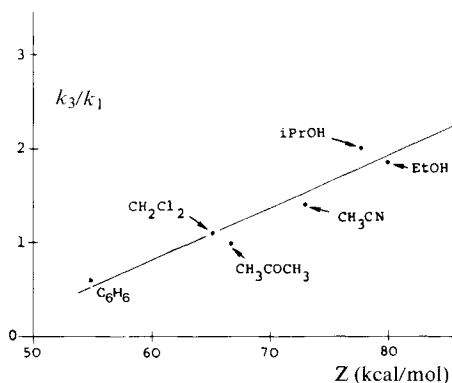
Fig. 2. k_3/k_1 vs. Z in various solvents.
