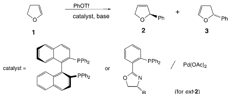
Scheme 1. The Intermolecular Asymmetric Heck Reaction of 2,3-Dihydrofuran with Phenyl Triflate. With PP ligands, the 2,3-dihydrofuran isomer predominates, but with PN ligands the 2,5-dihydrofuran isomer predominates.
