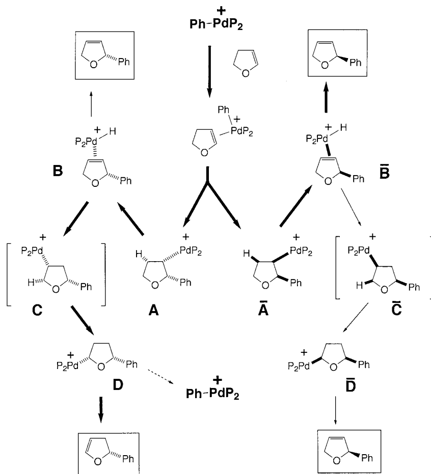
Scheme 2. Pathways for the Asymmetric Phenylation of 2,3-Dihydrofuran. The partitioning of the first-formed Pd–H complex B determines the course of reaction. With ( S )-BINAP as ligand, hydride return is the main pathway, giving the transient isomer C , which further rearranges to the most stable Pd–alkyl D , the precursor of the major product. On the minor enantiomer pathway, Pd–H complex B̄ preferentially partitions to the 2,5-dihydrofuran rather than further rearrangement through C̄ . Collapse to product through B or B̄ is the exclusive pathway when PN ligands are employed [7].
