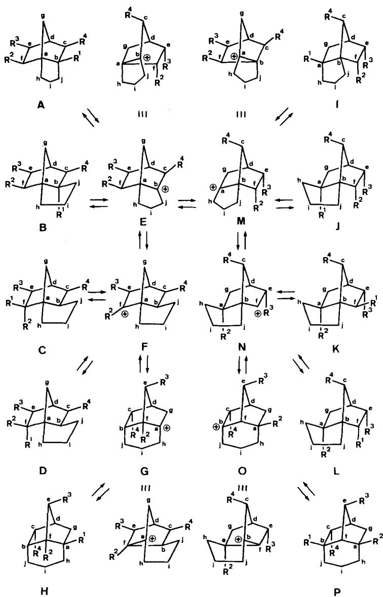
Scheme 3
