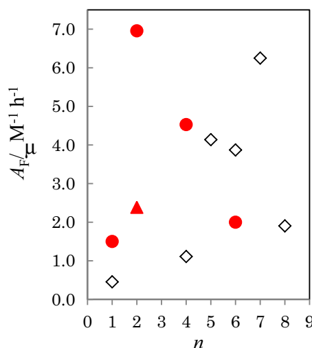
Fig. 2 Relationship between the A_F values and number of carbon atoms ( n ) in alkyl group on the alkylpyridinium (Apy) in 1a–1d (●), 1e–1j (◇), and 1k (▲)
