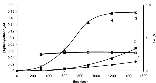
Figure 2. Kinetic data for hydrogenation of acetophenone catalyzed by 3 at 20 °C in \text{C}_6\text{H}_6 : [ 3 ] = 0.0003 M, [acetophenone] = 0.3 M; constant pressure of 5 atm \text{H}_2 (run 1, \blacklozenge ); [ 3 ] = 0.0003 M, [acetophenone] = 0.18 M, 5 atm \text{H}_2 (run 2, \blacksquare , corresponding ee values \square ); [ 3 ] = 0.0006 M, [acetophenone] = 0.18 M, 5 atm \text{H}_2 (run 3, \square ); and [ 3 ] = 0.0003 M, [acetophenone] = 0.18 M, 10 atm \text{H}_2 (run 4, \blacktriangle ).
