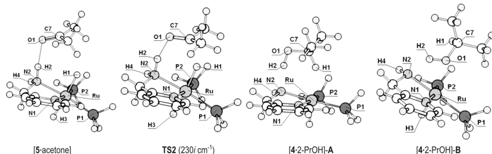
Figure 6. Optimized gas-phase structures of the model complexes and the transition state ( TS2 ) for the H 2 -hydrogenation of acetone with 5 as catalyst. Selected bond lengths (Å): [5·acetone] H1–C7 2.926, O1–C7 1.216, O1–H2 1.980, H2–N2 1.019, N2–Ru 2.165, Ru–H1 1.688, TS2 H1–C7 1.817, O1–C7 1.241, O1–H2 1.725, H2–N2 1.035, N2–Ru 2.139, Ru–H1 1.724, [4·2-PrOH]-A H1–C7 1.127, O1–C7 1.419, O1–H2 1.004, N2–H2 1.698, Ru–N2 2.052, Ru–H1 2.181, [4·2-PrOH]-B H1–C7 1.100, O1–C7 1.419, O1–H2 1.006, N2–H2 1.715, Ru–N2 2.094, Ru–O1 2.380.
