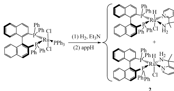
Scheme 5. Preparation of the Complex Ru(H)Cl(S-binap)(appH) ( 2 ) from RuCl 2 (S-binap)(PPh 3 )
