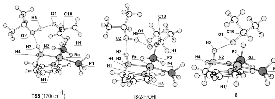
Figure 10. Optimized gas-phase structures of the model complexes and the transition state (TS5) for the alcohol-assisted ketone hydrogenation starting from 6 . Selected bond lengths (Å): TS5 H1–C10 1.786, C10–O1 1.241, O1–H5 1.658, O2–H2 1.869, [8·2-PrOH] Ru–O1 2.206, O1–C10 1.388, O1–H5 1.513, O2–H2 1.779, 8 Ru–O1 2.182, O1–H2 1.825, O1–C10 1.379.
