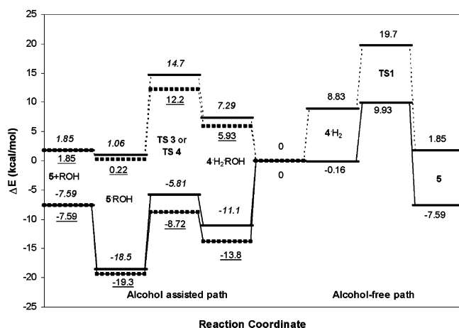
Figure 8. Comparison of the calculated energies for the alcohol-free \text{H}_2 splitting (from the middle to the right) and the alcohol-assisted \text{H}_2 splitting (from the middle to the left). The zero value at the middle is the starting relative energy of free 4 and \text{H}_2 for the alcohol-free path and free 4 , \text{H}_2 , and alcohol for the alcohol-assisted path. The \Delta G values (298.15 K, 1 atm) are corrected for the zero-point energies but uncorrected for translations and rotations. The solid line connects \Delta H , while the dashed line connects \Delta G values. The values for \text{R} = \text{C}_6\text{H}_5(\text{CH}_3)\text{CH}- are underlined, while those for \text{R} = (\text{CH}_3)_2\text{CH}- are in italics.
