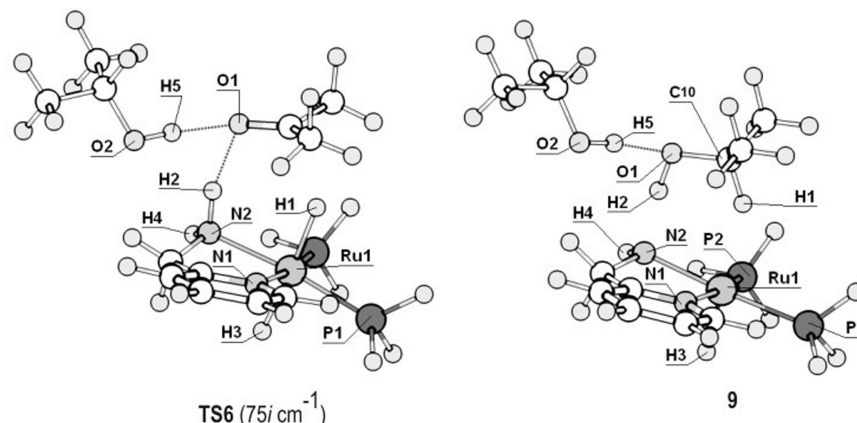
Figure 11. Optimized gas-phase structures of the model complexes and the transition state (TS6) for the alcohol-assisted ketone hydrogenation starting from 7 . Selected bond lengths (Å): TS6 H1–C10 2.087, H2–O1 1.882, H5–O1 1.859, O1–C10 1.235, 9 H1–C10 1.125, O1–C10 1.400, O1–H2 1.033, H2–N2 1.581, H5–O1 1.811.
