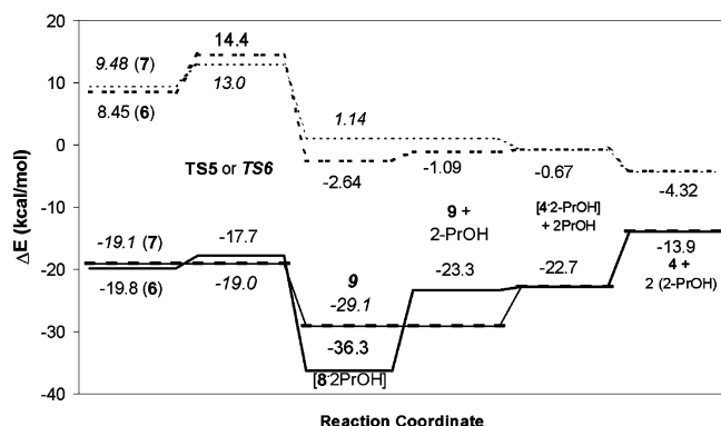
Figure 12. Part of the energy profile for the alcohol-assisted hydrogenation of acetone, starting from 6 or 7 (Figure 9). The solid lines connect the \Delta H , while the dashed lines connect the \Delta G values. The energy values for the cycle starting with 6 are in normal font, while those for the cycle starting from 7 are in italics. The energies are relative to free 4 , acetone, 2-propanol, and H_2 for easier comparison with the energy profiles of Figure 8. The reaction sequence ends with two free 2-propanol and the regenerated free amido 4 .
