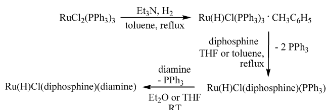
Scheme 4. General Preparation of the Complexes trans -RuHCl(diphosphine)(diamine)
