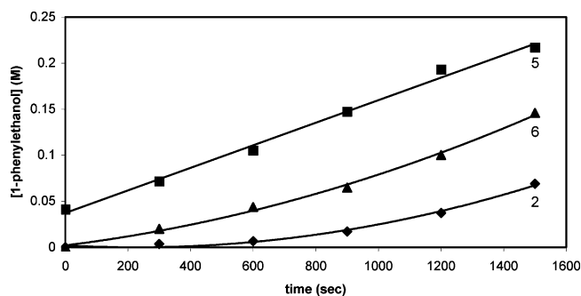
Figure 3. Data for the catalytic hydrogenation of acetophenone (0.18 M) in \text{C}_6\text{H}_6 at 20 °C with [\mathbf{3}] = 0.0003 M under 5 atm of \text{H}_2 and no additive (run 2, ◆), rac -1-phenylethanol added (0.04 M, initial concentration) (run 5, ■), and 2-propanol added (0.06 M) (run 6, ▲).
