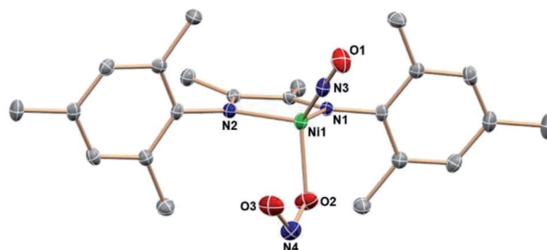
Fig. 2 ORTEP representation of the molecular structure (50% probabilities) of the nonhydrogen atoms of (DIM)Ni(NO)(ONO) showing selected atom labelling (unlabelled atoms are carbon). Selected structural parameters: Ni1–N3, 1.637(2); Ni1–O2, 1.9952(19); Ni1–N2, 2.0075(19); Ni1–N1, 2.0204(19); O1–N3, 1.176(3); O2–N4, 1.280(3); O3–N4, 1.228(3); N4–O2–Ni1, 118.25(16); O1–N3–Ni1, 175.5(2).
