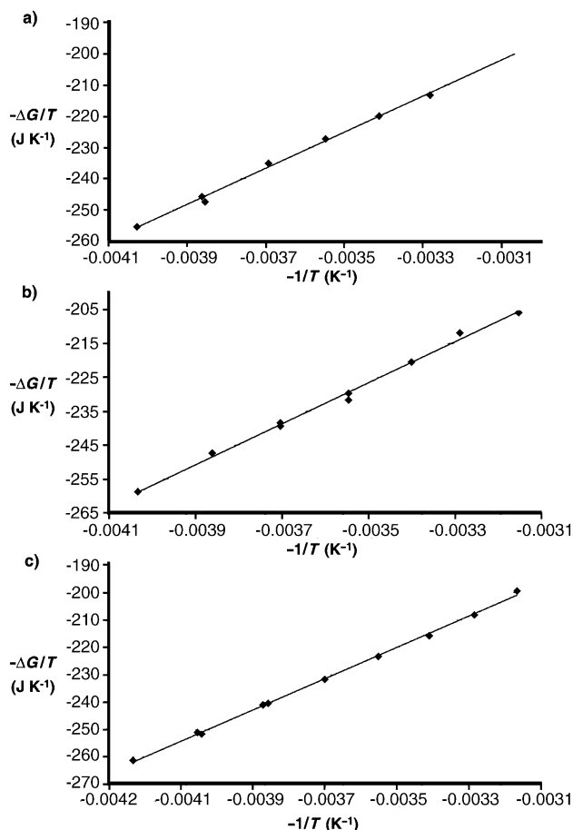
Figure 7. Eyring plots created from the data in Tables 2–4 for the degenerate rotaxanes a) 1 – 4 PF 6 , b) 3 – 4 PF 6 , and c) 5 – 4 PF 6 . The values for \Delta H^\ddagger and \Delta S^\ddagger were obtained from the slopes and intercepts of these plots, respectively, and are given in Table 5.
