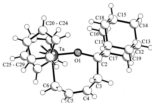
Fig. 1. A view of the molecular structure of complex 2a (cation only, with unsystematical atom numbering scheme). Selected bond lengths (Å) and angles ( ^\circ ): Ta–O1 1.846(2), O1–C2 1.443(3), C2–C11 1.542(4), C2–C17 1.532(4), C2–C3 1.556(4), C3–C4 1.501(5), C4–C5 1.328(5), C5–C6 1.483(5), Ta–C6 2.247(3); O1–Ta–C6 90.15(11) , Ta–O1–C2 160.76(17) , O1–C2–C3 103.1(2) , O1–C2–C17 109.6(2) , O1–C2–C11 108.7(2) , C2–C3–C4 114.0(2) , C3–C4–C5 125.4(3) , C4–C5–C6 126.1(3) , C5–C6–Ta 108.5(2) .
