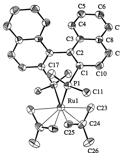
Fig. 1. The ORTEP plot of Ru(( R )-binap)( \eta^3 -Me-allyl) 2 3 . Thermal ellipsoids for non-hydrogen atoms are drawn at 33% probability (some of the phenyl carbons have been omitted for clarity). A C 2 axis rotates the labeled half of the molecule into the non-labeled half (e.g. P(1) reflects into P(1')).
