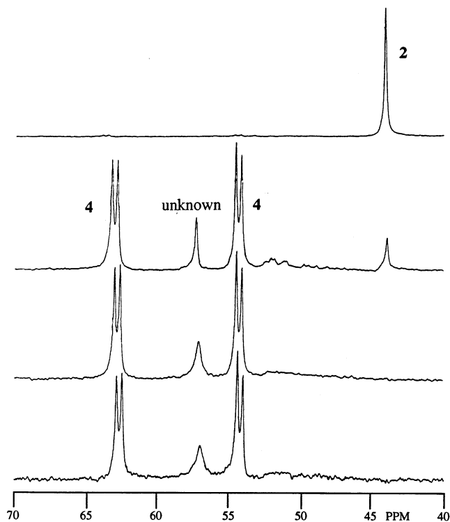
Fig. 3. 31 P{ 1 H}-NMR spectra (121.42 MHz, 20°C) of Ru(dppb)(η 3 -Me-allyl) 2 2 in CDCl 3 with: (a) no added HCl, (b) one equivalent HCl, (c) two equivalents HCl, and (d) three equivalents HCl. [Ru-Cl(dppb)] 2 (μ-Cl) 2 , 4 . δ A 63.5, δ B 54.3 (J AB 46.9 Hz). For the dimeric bromo and iodo species the corresponding data are δ A 65.2, δ B 55.6 (J AB 44.3 Hz) and δ A 70.1, δ B 55.6 (J AB 39.9 Hz), respectively [17].
