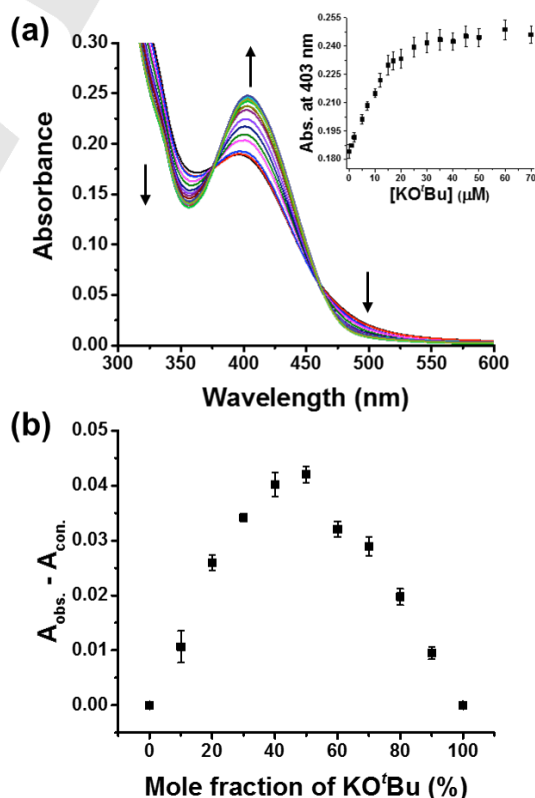
Figure 4. (a) UV-Vis spectra of L7-Ni (20 \mu M) in the presence of varying amounts of KOt-Bu (0 ~ 70 \mu M) in THF. Inset: Plot of absorbance at 403 nm versus concentration of KOt-Bu. (b) Job plot for binding mode between L7-Ni and K^+ ions in THF. A_{obs} : Absorbance of L7-Ni at 403 nm with varying amounts of KOt-Bu; [L7-Ni] + [KOt-Bu] = 40 \mu M, A_{con} : Absorbance of L7-Ni (40 to 0 \mu M) at 403 nm without KOt-Bu.
