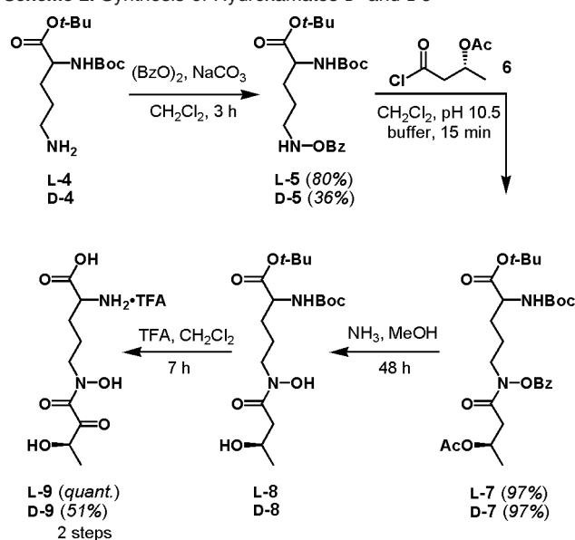
Scheme 2. Synthesis of Hydroxamates D- and L-9 a
