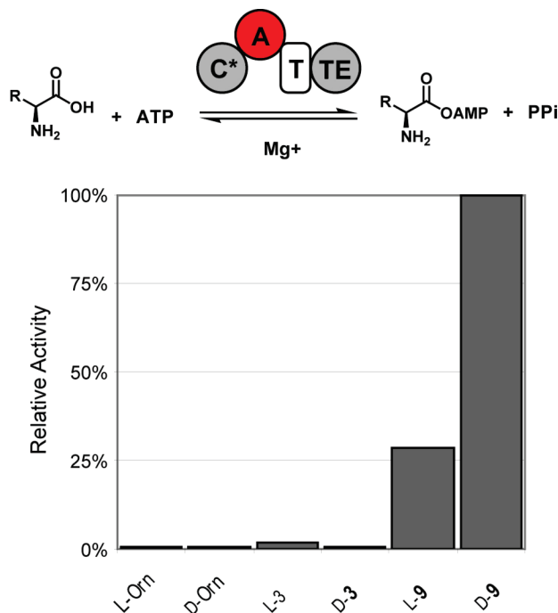
Figure 6. Relative activities of the VbsS adenylation (A) domain with L- and D-Orn, L- and D-3 and L- and D-9 as assessed by ATP-[ ^{32} P]PPi exchange assays.
