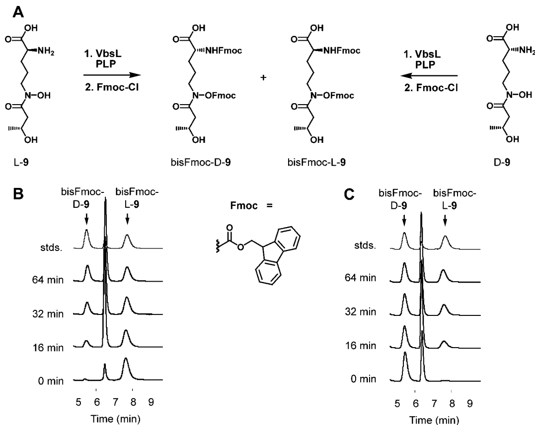
Figure 5. Characterization of VbsL as a PLP-dependent epimerase. (A) Schematic of the VbsL-catalyzed racemization of N 5 -(( R )-3-hydroxybutyryl)- N 5 -hydroxy-L- or D-ornithine (L-9 or D-9) and proposed structure of the Fmoc-derivatized products (bisFmoc-L-9 and D-9). (B) Chiral HPLC traces (263 nm) showing racemization of L-9 (1 mM) resulting from incubation with VbsL (500 nM), PLP (50 μM) and pH 7.75 HEPES (50 mM) followed by derivatization with Fmoc-Cl. (C) Chiral HPLC traces (263 nm) showing racemization of D-9 (1 mM) resulting from incubation with VbsL (500 nM), PLP (50 μM) and pH 7.75 HEPES (50 mM) followed by derivatization with Fmoc-Cl. Peaks corresponding to bisFmoc-D-9 appear at t R 5.4 min and bisFmoc-L-9 at t R 7.6 min. Peak at t R 6.4 min is an artifact of Fmoc-Cl decomposition in aqueous solution.
