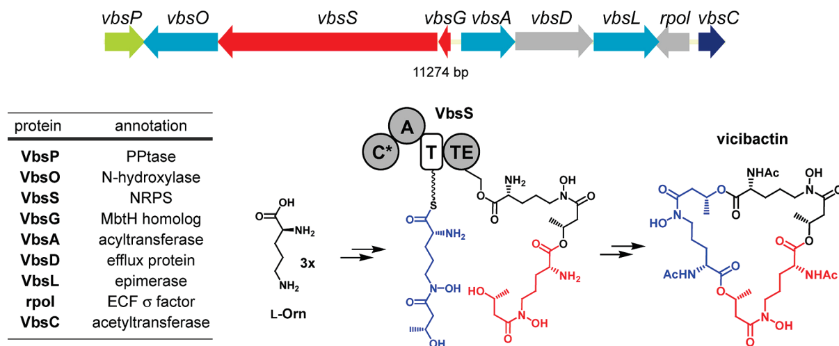
Figure 2. Vicibactin gene cluster and annotated protein functions. The multidomain NRPS, VbsS, is thought to be the central catalyst responsible for trimerization of the functionalized ornithine monomer. The N-terminal condensation domain (marked C*) of VbsS lacks required conserved residues in the active site and is thought to be inactive. (A = adenylation domain, T = thiolation domain, TE = thioesterase domain.)
