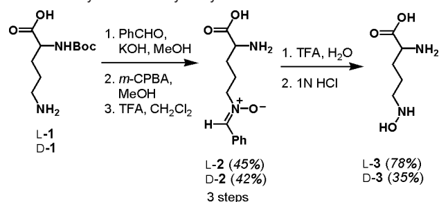
Scheme 1. Synthesis of Hydroxylamines L- and D-3 a
