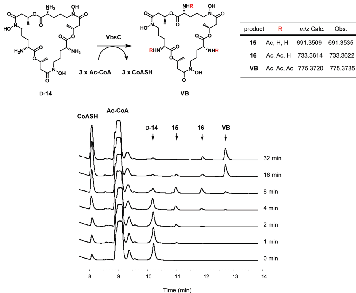
Figure 7. Characterization of VbsC as a CoA-dependent desacetyl-D-vicibactin N^2 -acetyltransferase. (A) Schematic of the VbsC-catalyzed, triacetylation of desacetyl-D-vicibactin ( D-14 ) with 3 equiv of acetyl-CoA and ESI-HRMS m/z data of purified products. (B) HPLC traces (220 nm) showing the time-dependent appearance of mono-, di- and triacetylated products resulting from the incubation of D-14 (1 mM) and acetyl-CoA (4 mM) with VbsC (10 \mu M) in pH 7.75 HEPES (50 mM). Peaks corresponding to CoASH appear at t_R 8.1 min, Acetyl-CoA at t_R 9.1 min, D-14 at t_R 10.2 min, monoacetylated D-15 at t_R 11.0 min, diacetylated D-16 at t_R 11.9 min, and VB at t_R 12.8 min.
